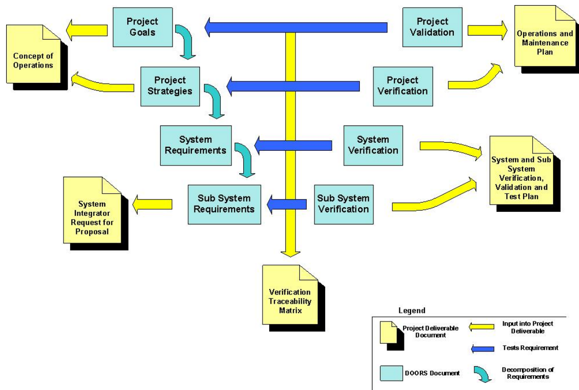
Figure 4 Relationship between DOORS documents and deliverables
