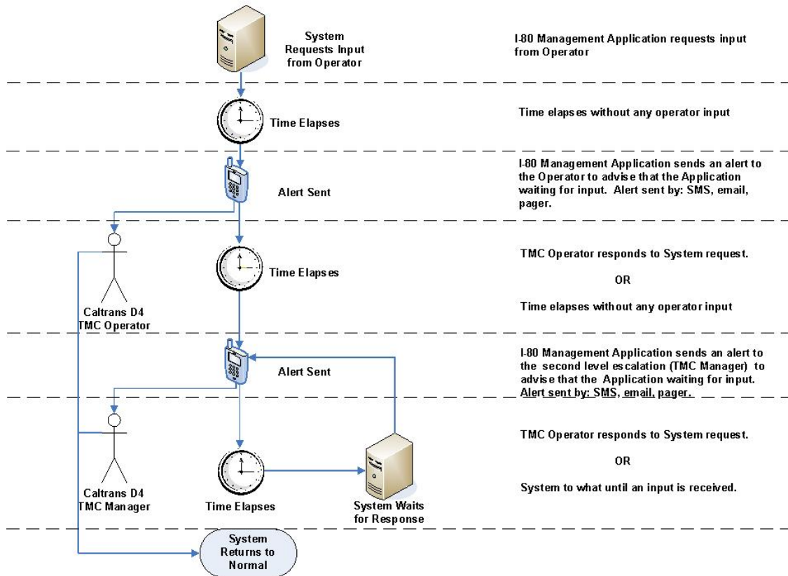
Figure 3 Example Hybrid Sequence Diagram
