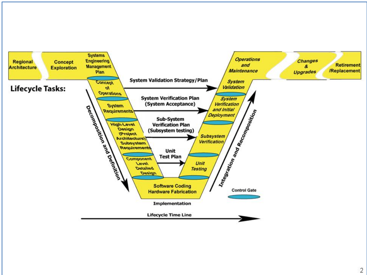
Figure 2 System Engineering "winged vee"
